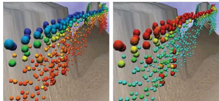
Figure 2: On the left is view with glyph size being mapped to chlorophyll levels and color being mapped to salinity levels. Smaller sized glyphs correspond to lower levels of chlorophyll, while blues correspond to lower salinity values. On the right is a view of the glyphs with both size and color mapped to chlorophyll.
