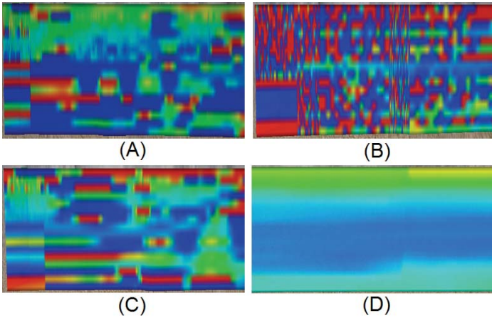
Figure 5: A comparison of radial basis function interpolation with different basis functions. (A) shows the result of a multiquadric (\sqrt{r^2 + B^2}) basis function. (B) shows a polyharmonic spline (r^{n-1}) . (C) shows a Gaussian (e^{-Br^2}) basis function. (D) shows the shifted log (\sqrt{\log_{10}(r^2 + B^2)})
