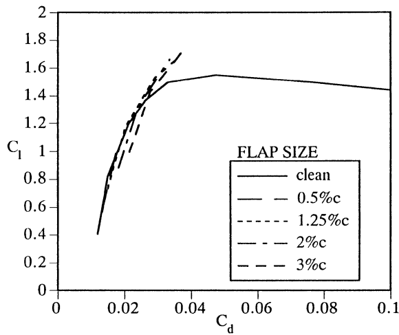
Fig. 11. Effect of Gurney flap size on drag polars; NACA 4412 airfoil, Re_c = 1.64 \times 10^6 .
