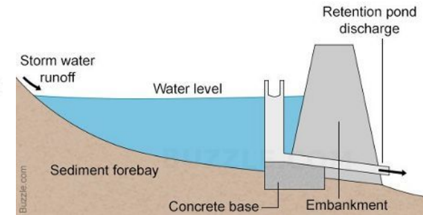
Storm Water Retention Pond and Control Structure
