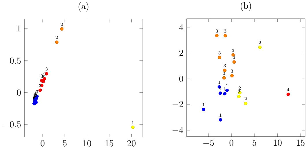
Figure 7.2: Clusters based on (a) code smell/metric and (b) framework. Each color/number represents a unique cluster. The units of the axes represent a linear combination of the feature set produced by Principle Component Analysis (PCA).
