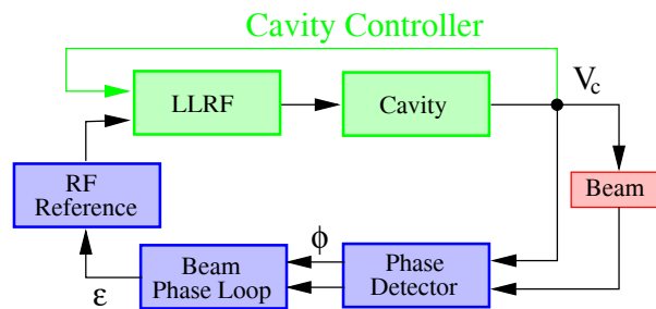
Figure 1: Simplified block diagram of the RF system with Beam Phase Loop.
