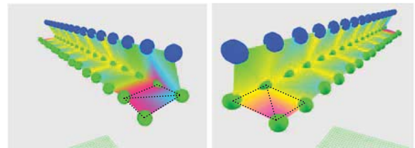
Figure 10 - Unrealistic Forces. Two panels (left, right) show bending force views of two sides of the same experiment on a v-beam with pinned vertices. The forces are asymmetric due to the underlying triangulation of the mesh. The black lines indicate triangle edges.
