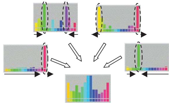
Figure 2 - The ITS histogram compression algorithm.
