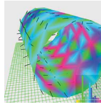
Figure 7 - Visible force vectors and force-based vertex pseudo-coloring
