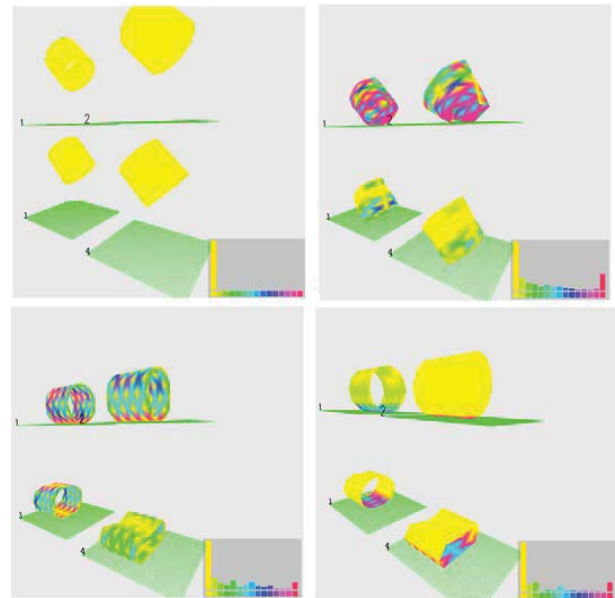
Figure 8 - The progression of forces in four dropped cylinders with varying internal force contributions.
