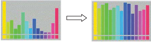
Figure 3 - Histogram equalization
