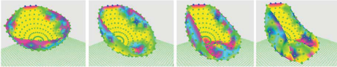
Figure 1 - Simultaneous Experiments. A pseudo-colored hollow cloth bowl with three pinned vertices is simulated collapsing under the force of gravity. Each image depicts the same moment in time for the same mesh, with decreasing membrane and bending energy constants, from left to right.
