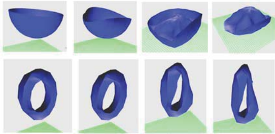
Figure 5 - Two mesh experiments: A falling half sphere impacting an invisible cube and a ring, pinned at a single point, shown at the same moment in time, with decreasing membrane and bending force constants.
