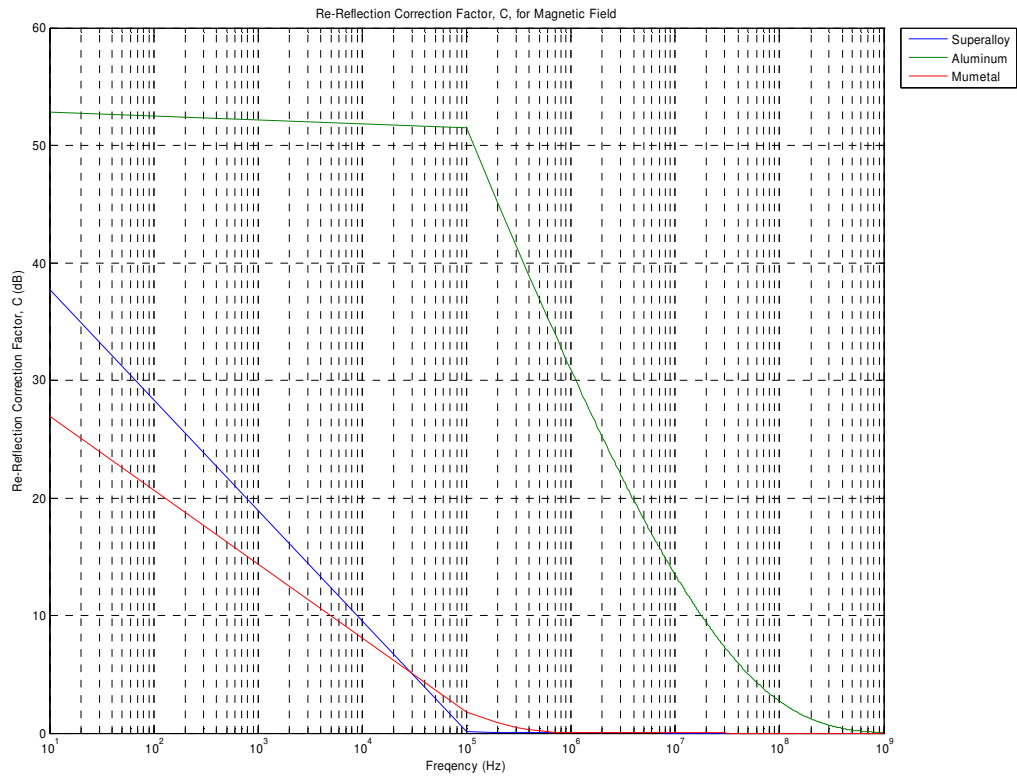
Figure 14. Re-Reflection Correction Factor for Magnetic Field
