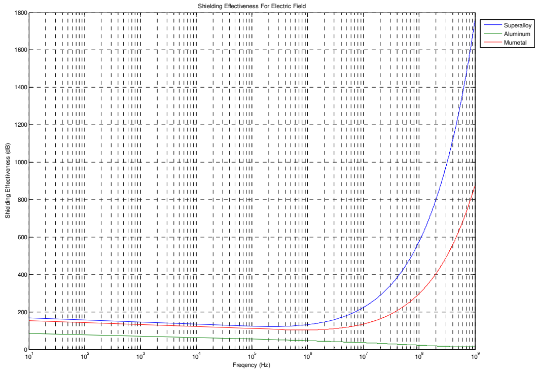
Figure 18a. Shielding Effectiveness for Electric Field
