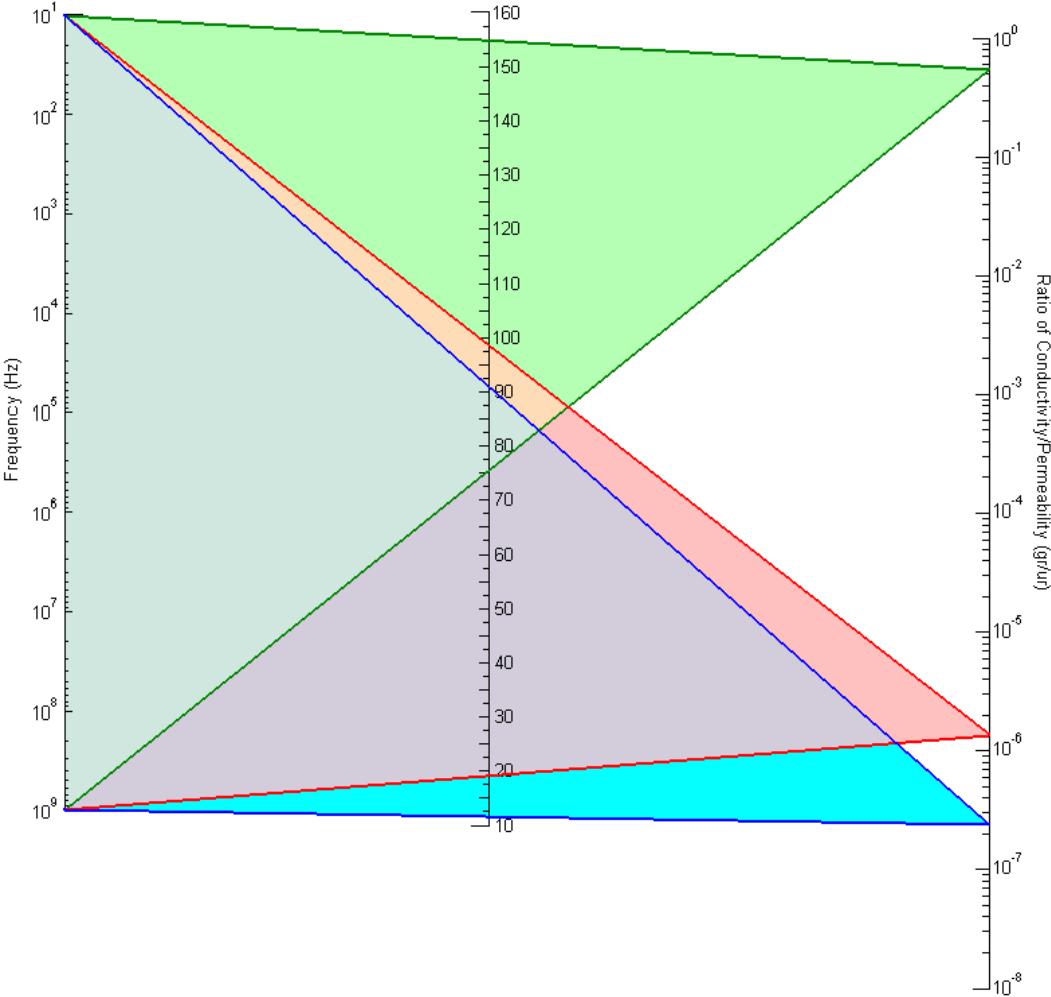
Figure 10. Nomograph to Calculate the Reflection Loss for plane Wave
