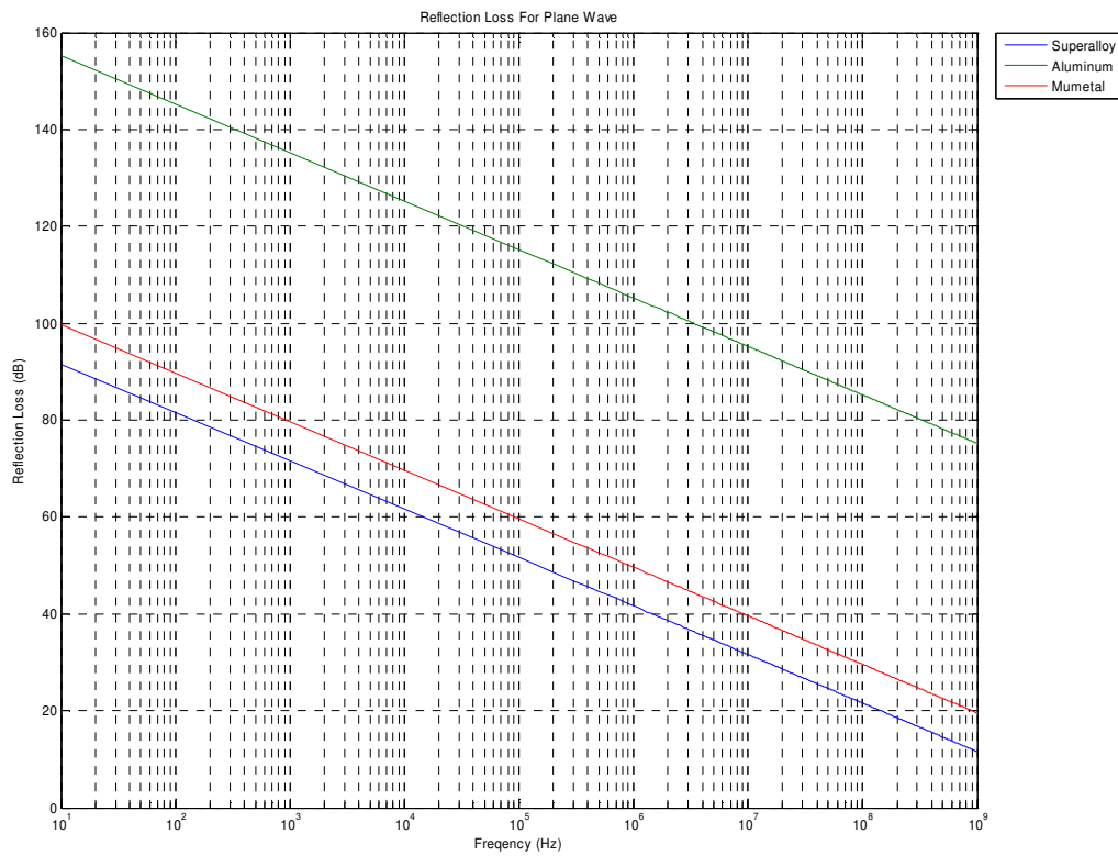
Figure 9. Reflection Loss for Plane Wave
