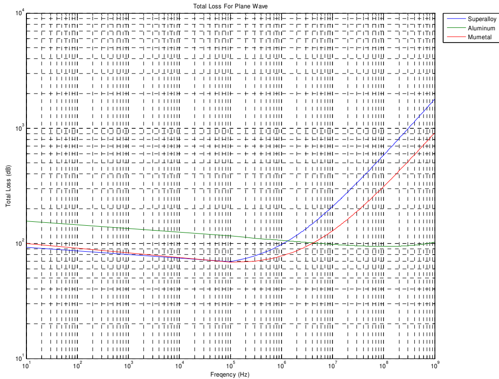
Figure 13. Total Loss for Plane Wave
