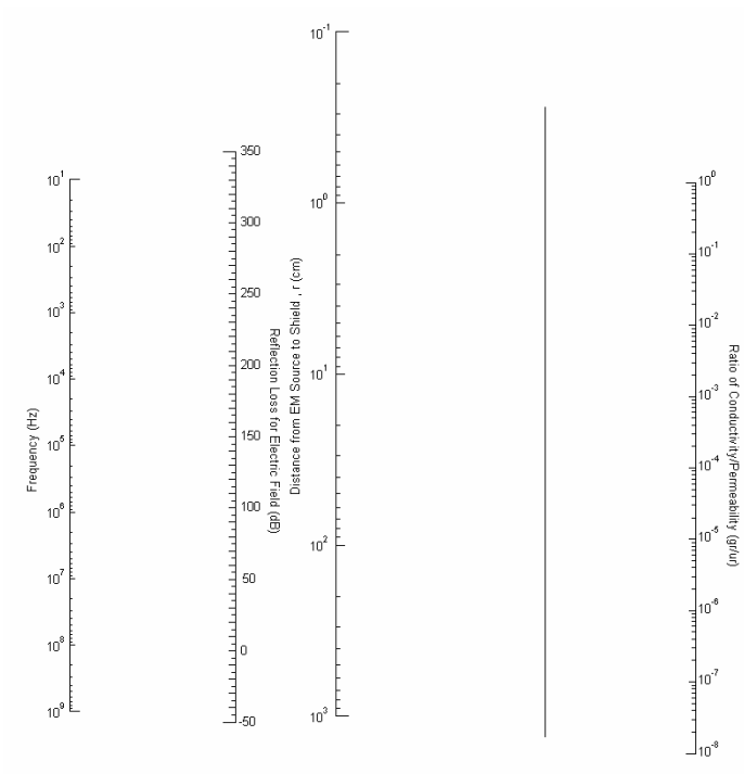
Figure 2b. Reflection Loss Nomograph for Electric Field
