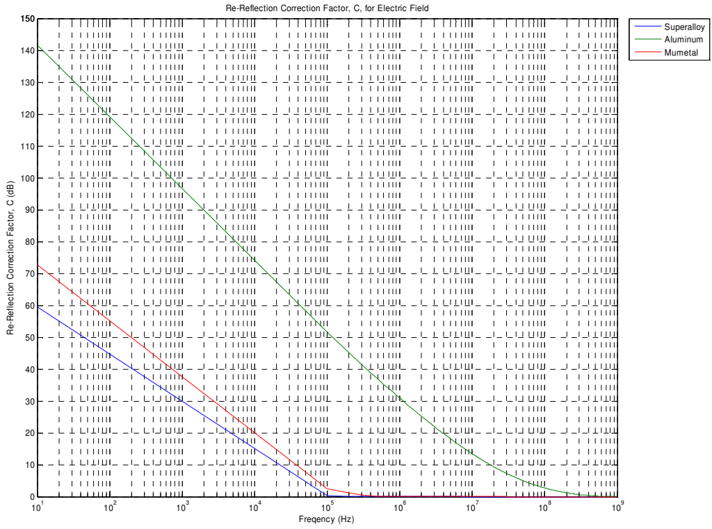
Figure 15. Re-Reflection Correction Factor for Electric Field
