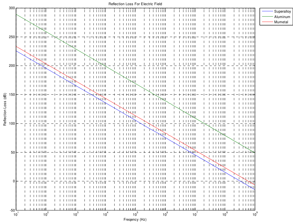
Figure 7. Reflection Loss for Electric Field produced by Matlab
