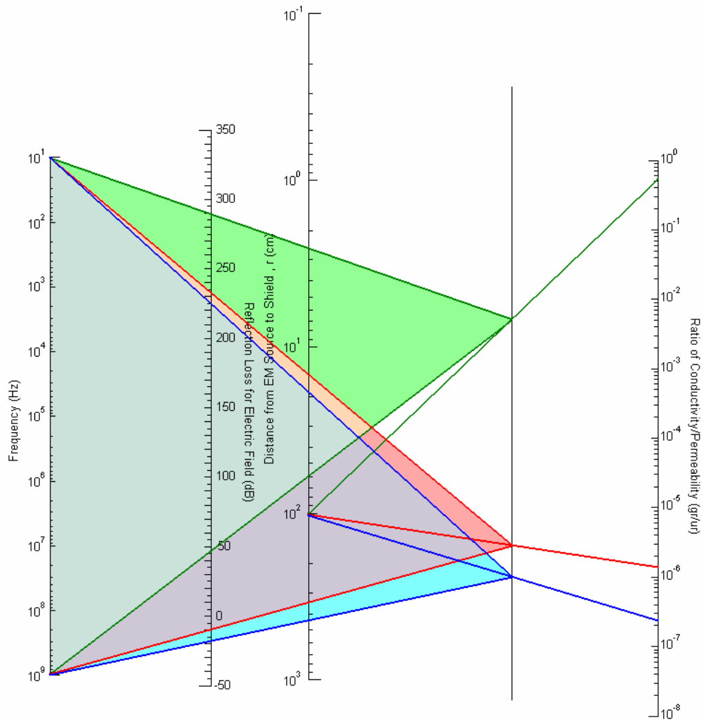
Figure 8. Nomograph to Calculate the reflection Loss for Electric Field
