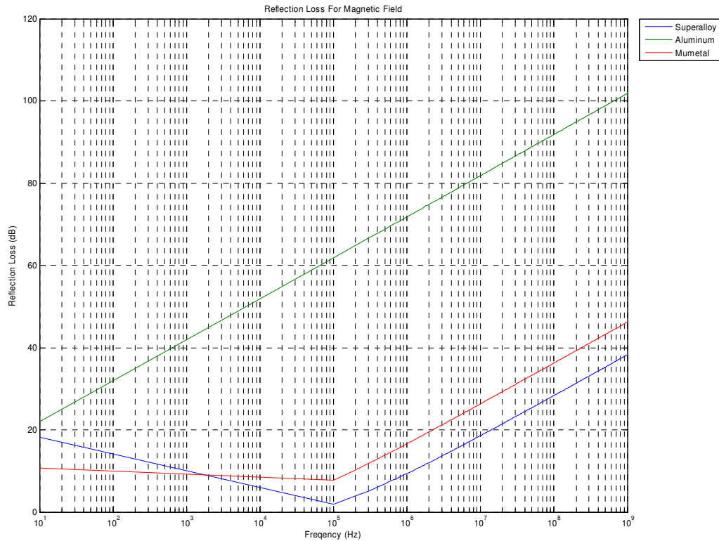
Figure 5. Reflection Loss for Magnetic Field produced by Matlab
