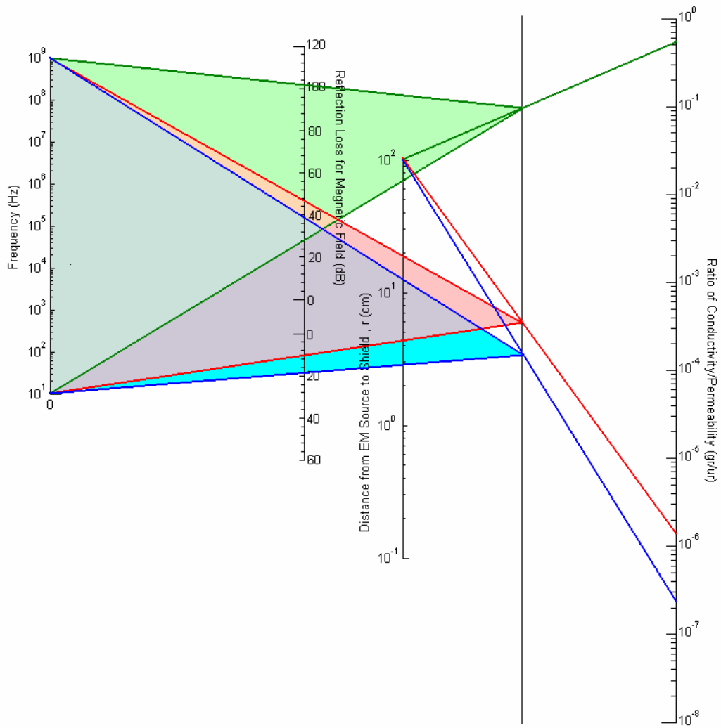
Figure 6. Nomograph to Calculate the Reflection Loss for Magnetic Field
