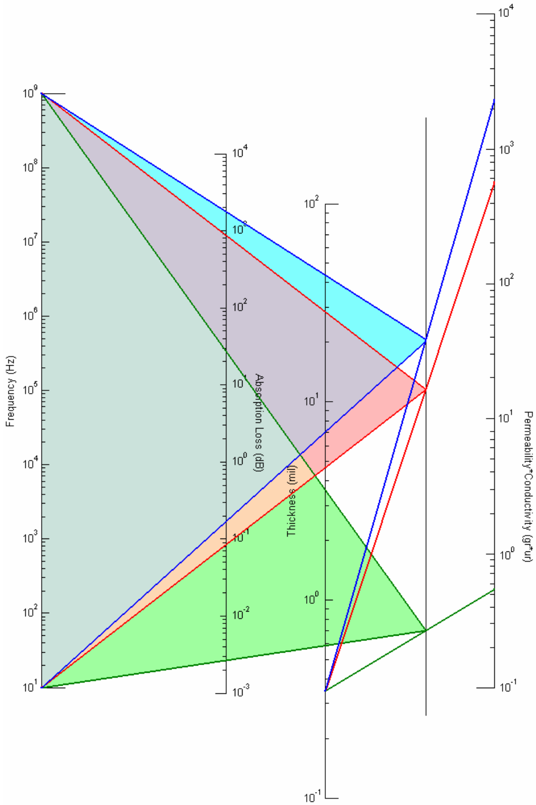
Figure 4. Nomograph to Calculate the Absorption Loss for Magnetic Field, Electric Field, and Plane Wave
