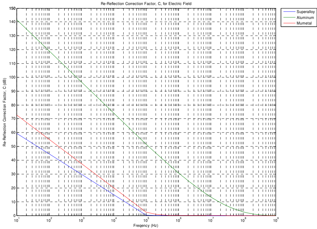
Figure 16. Re-Reflection Correction Factor for Plane Wave
