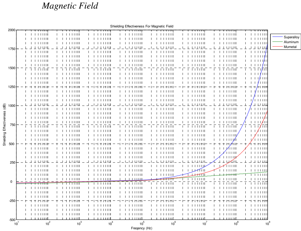
Figure 17a. Shielding Effectiveness for Magnetic Field
