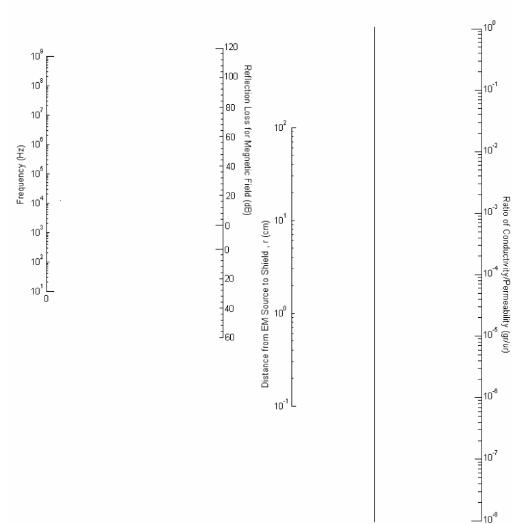
Figure 2a. Reflection Loss Nomograph for Magnetic Field
