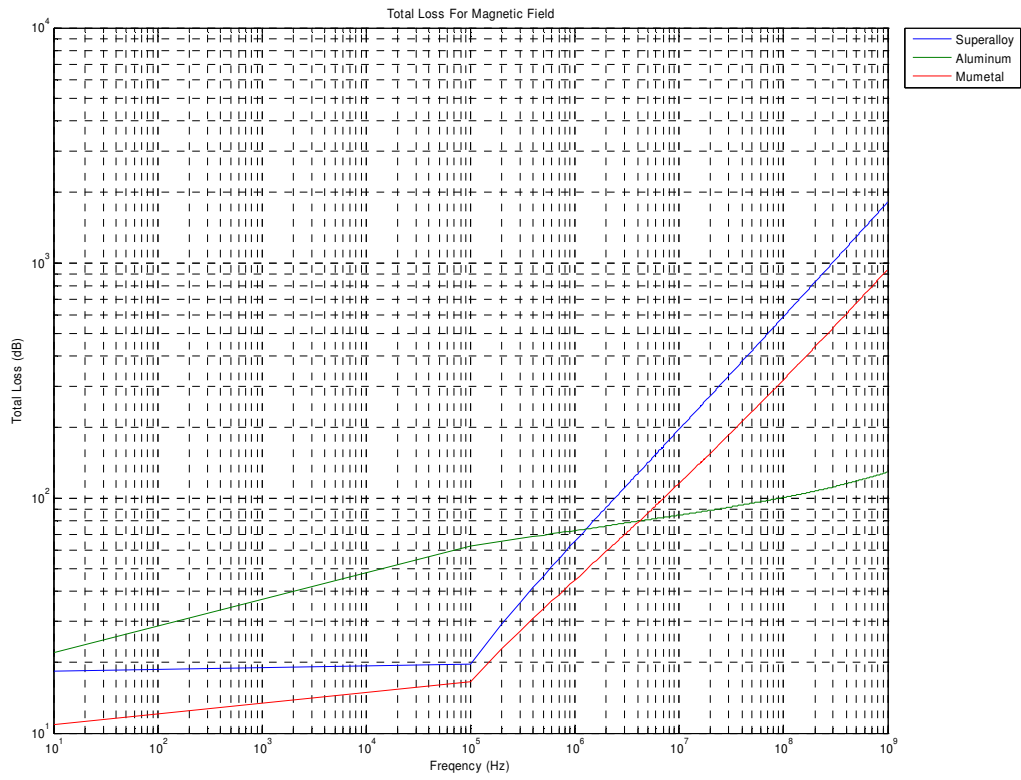
Figure 11. Total Loss for Magnetic Field
