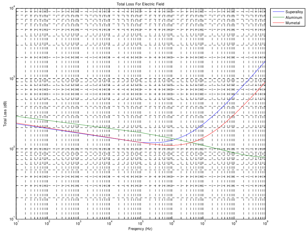
Figure 12. Total Loss for Electric Field
