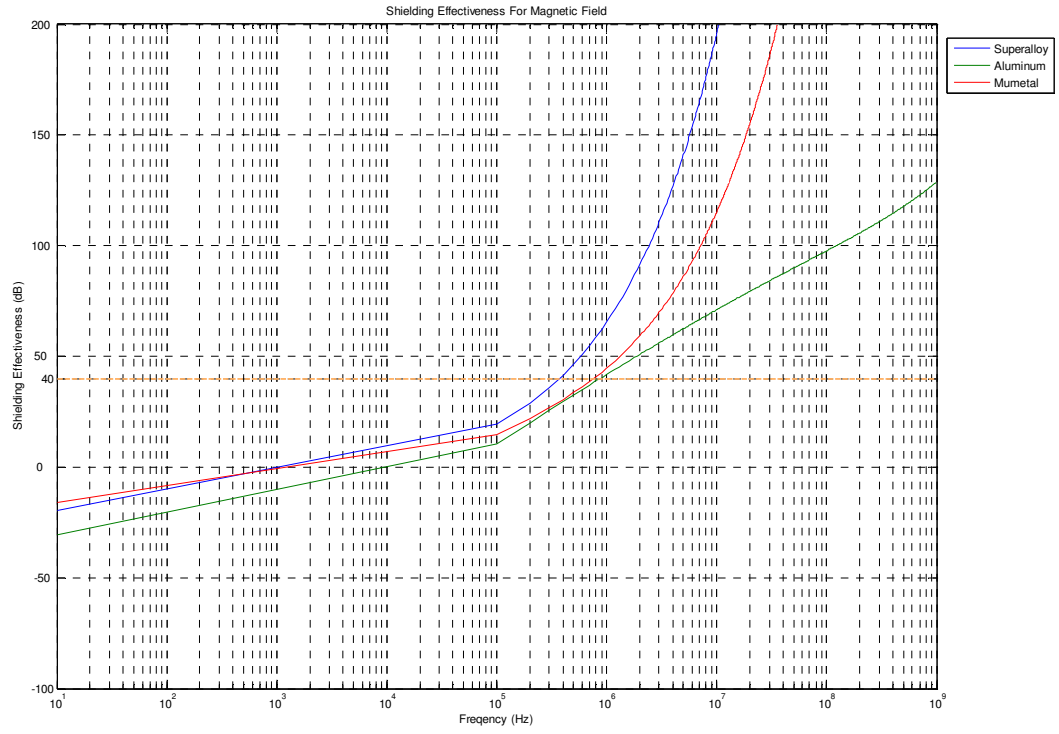
Figure 17b. Shielding Effectiveness for Magnetic Field Up to 200 dB
