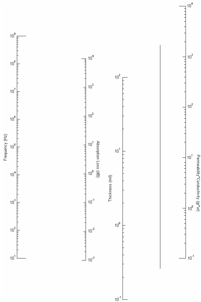
Figure 1. Nomograph for Absorption Loss
