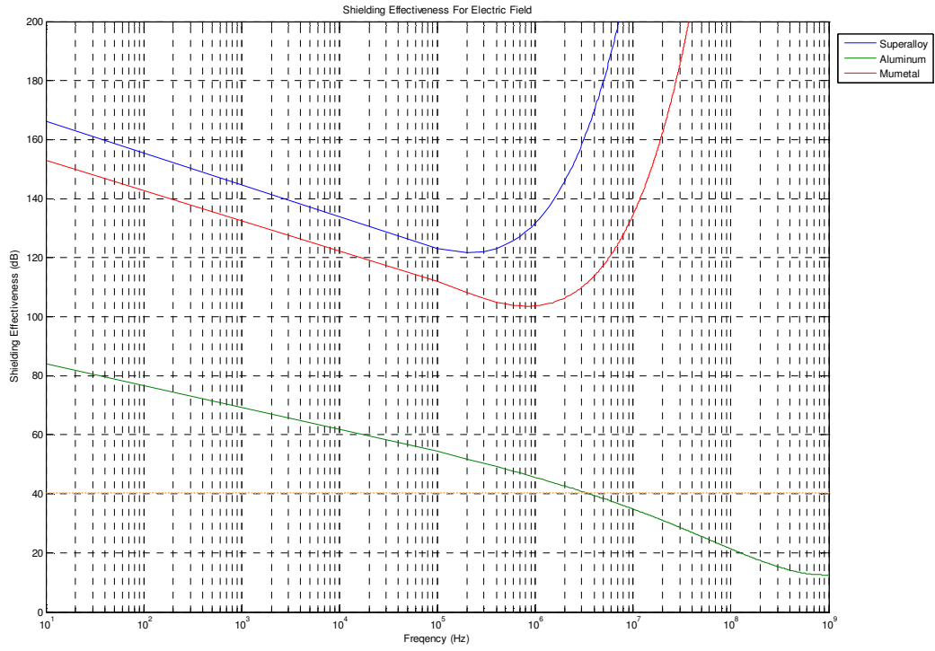
Figure 18b. Shielding Effectiveness for Electric Field Up to 200 dB
