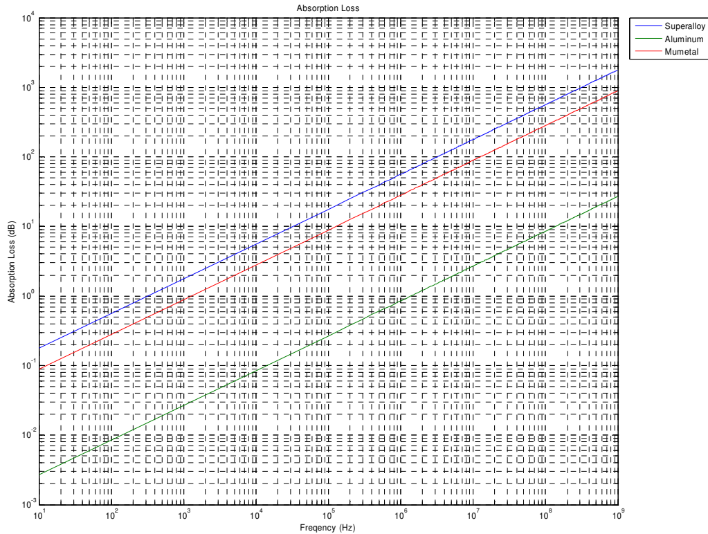
Figure 3. Absorption Loss for Magnetic Field, Electric Field, and Plane Wave produced by Matlab
