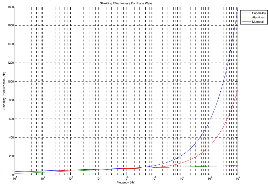
Figure 19a. Shielding Effectiveness for Plane Wave
