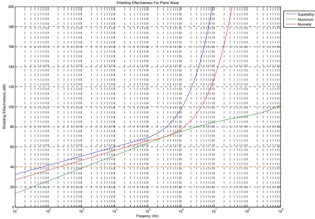
Figure 19b. Shielding Effectiveness for Plane Wave Up to 200 dB
