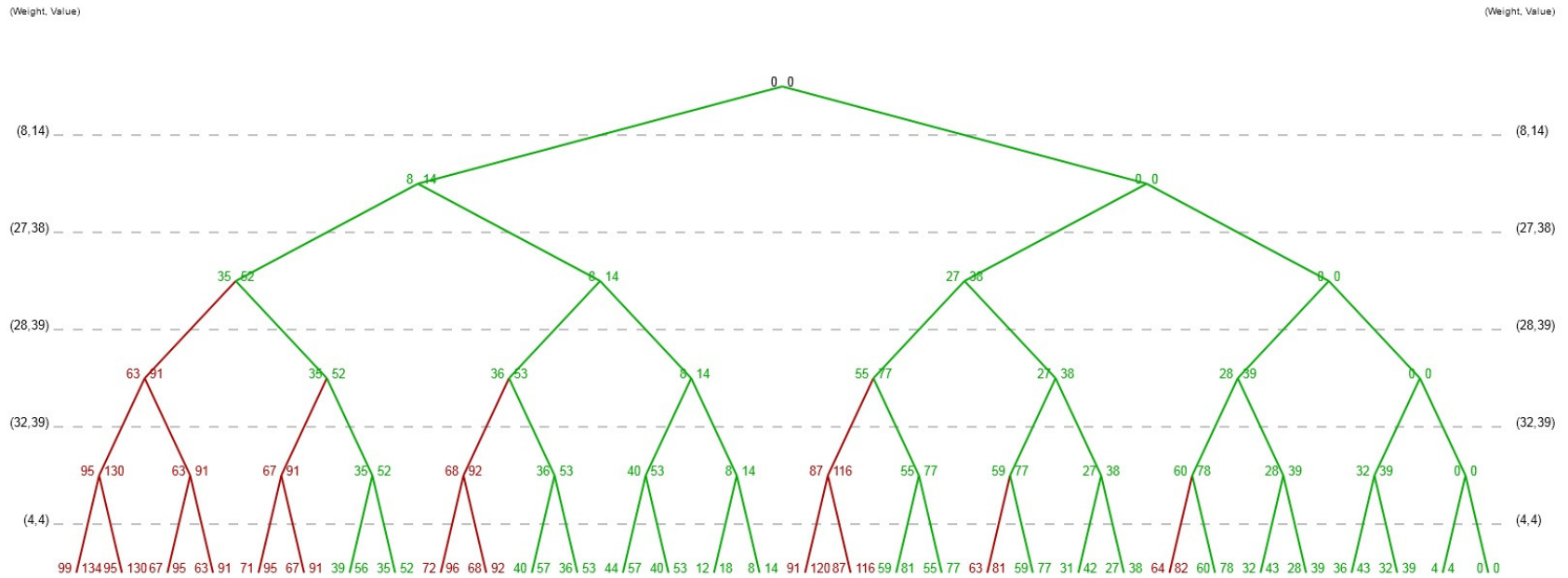
Figure 3: Branch & Bound Example
