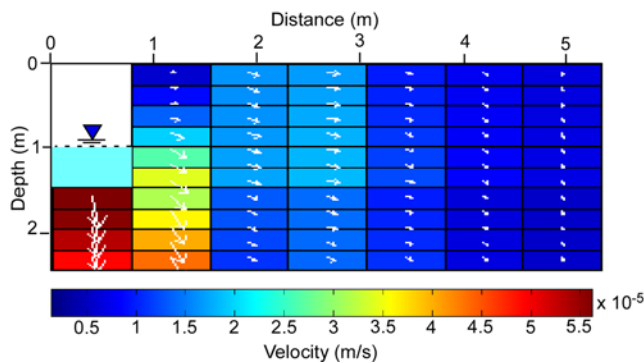
Figure 4. Reconstruction of the Darcy velocity from the self-potential data of Suski et al. [2006] ( R^2 = 0.98 ) using an a prior model.
