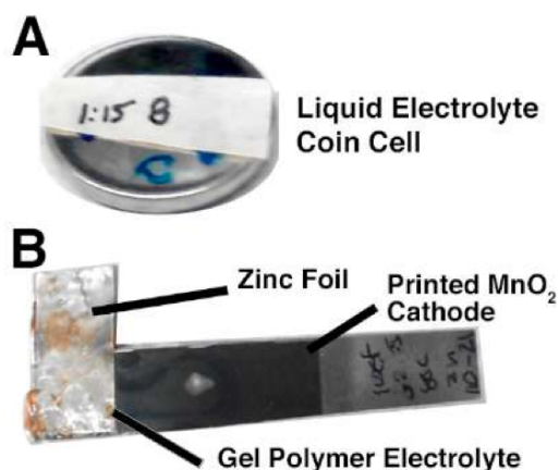
Figure 2. Test cell form factors. A) Coin cell containing liquid electrolyte (no PVDF-HFP gel component); B) Sandwich cell.
