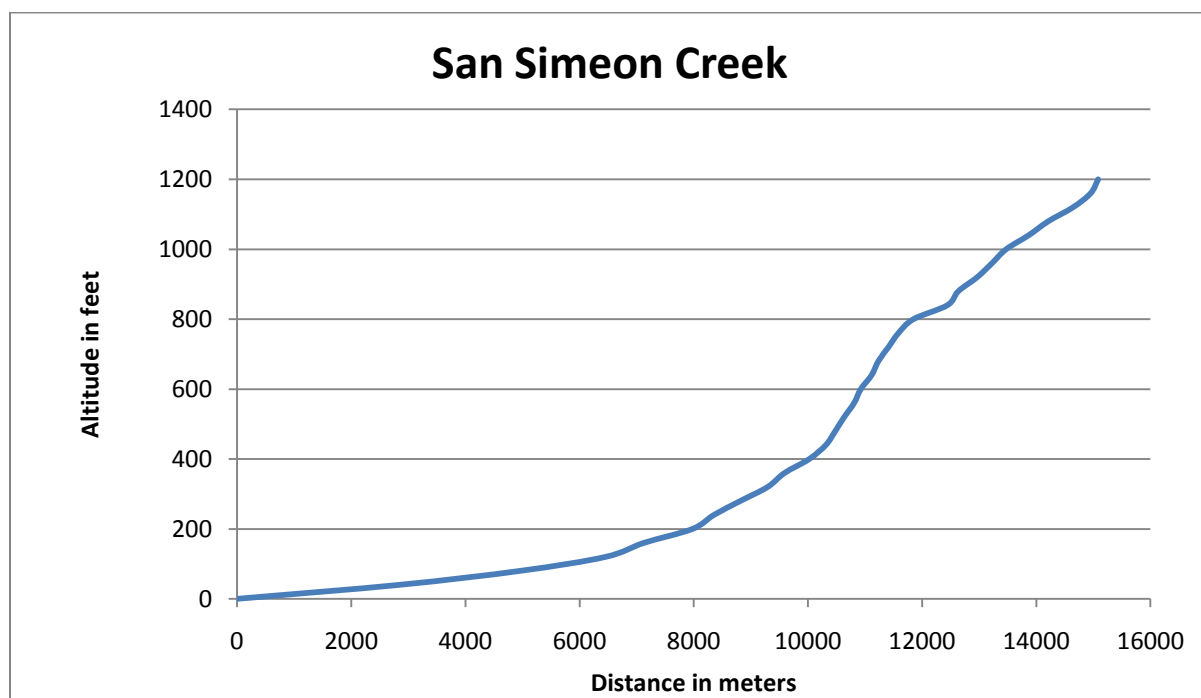
Fig. 7 Stream profile of San Simeon Creek.
