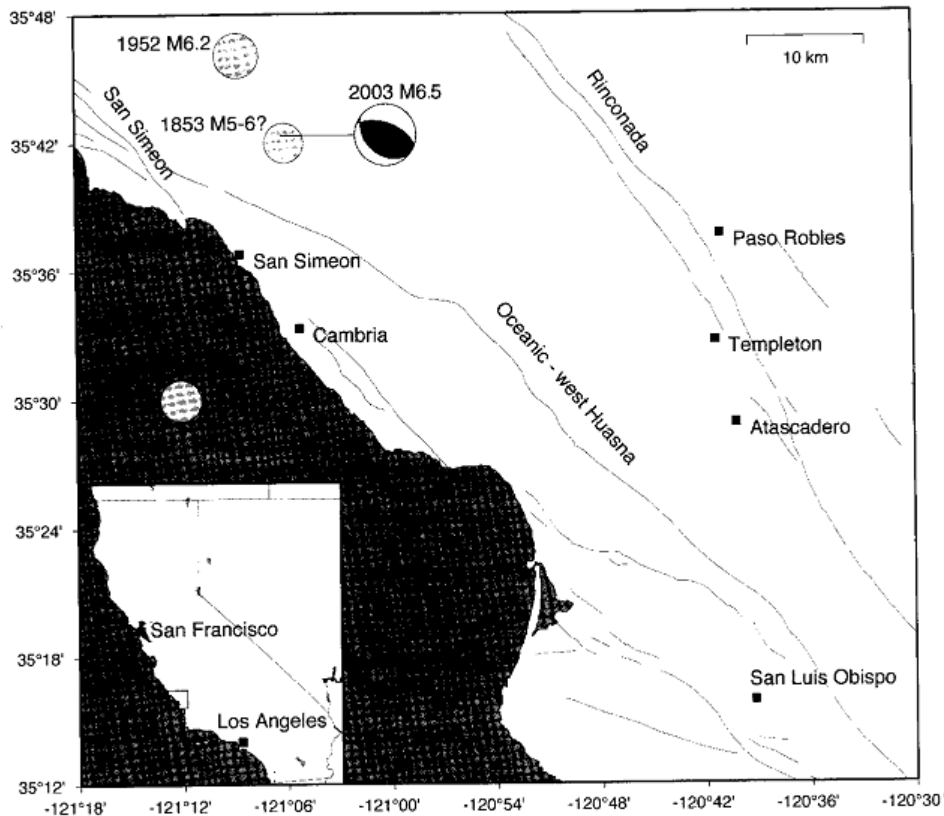
Fig. 4 A map of the hypocenter of the 2003 M 6.5 San Simeon earthquake with moment-tensor solution (Hardebeck, 2004).
