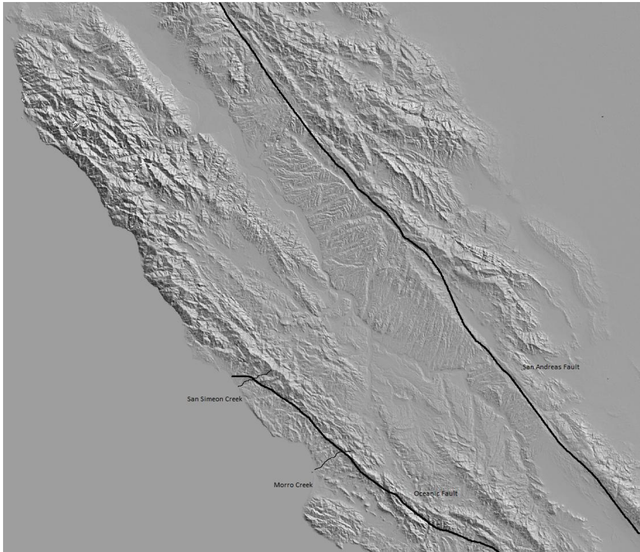
Fig. 1 A Digital Elevation Model of California's Central Coast.
