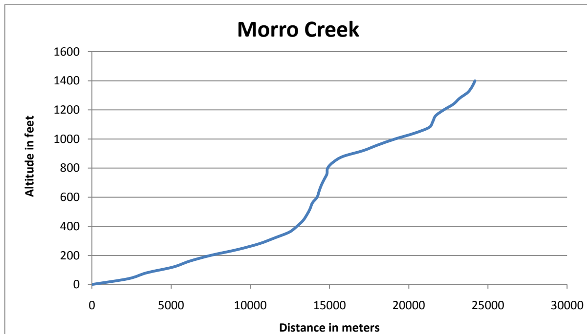
Fig. 6 Stream Profile of Morro Creek.
