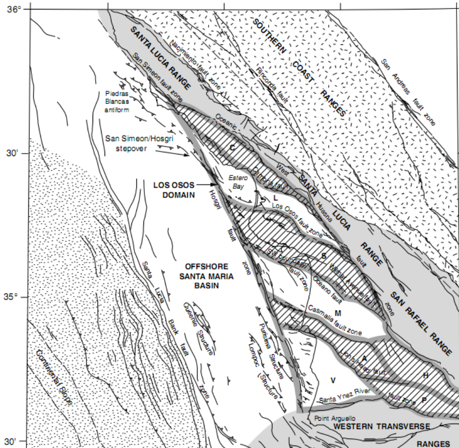
Fig. 3 A map of the Los Osos Domain (McLaren and Savage, 2001).
