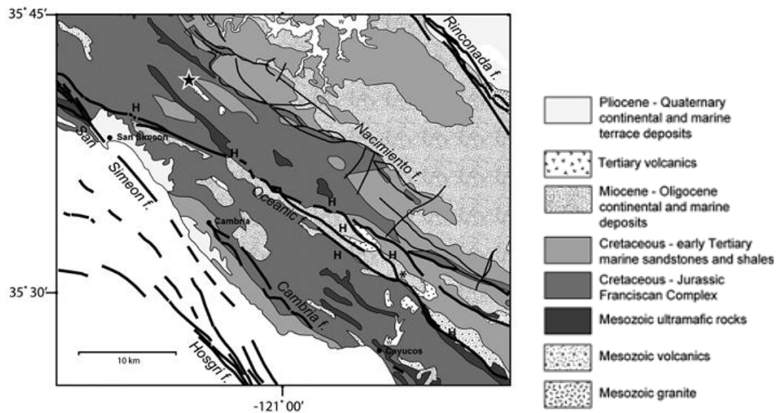
Fig. 2 Basement rock map west of the San Andreas Fault (McLaren et. al. 2008) the star is the San Simeon earthquake epicenter.
