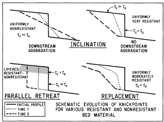
Fig. 5 Models of knickpoint evolution. \tau_c is critical bottom shear stress needed to initiate erosion. \tau_0 actual bottom shear stress. (Gardner, 1987).
