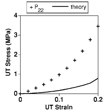
Fig. 5 Prediction of the eight-parameter model that does not include the traction-free boundary condition equations (8-PAR-B) for the uniaxial tension (UT) response in the 2 direction. The predictions for the UT response in the 1 and 3 directions and the UCC response in the 1 direction are similar to those of the 8-PAR model shown in Fig. 3.
