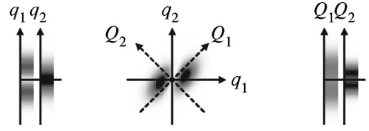
Fig. 7. Probability density for \hat{q}_1|0,0\rangle .
