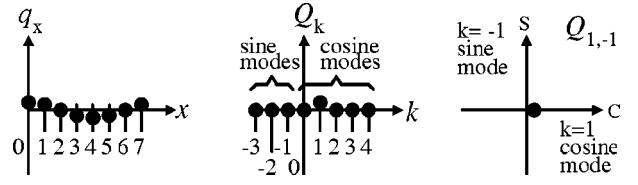
Fig. 9. The coordinate axes used to plot the eight-particle lattice.
