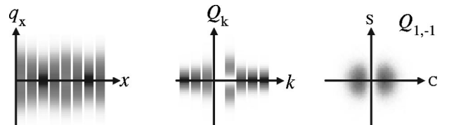
Fig. 13. The quantum mechanical lattice with one k=1 phonon, \hat{A}_1^\dagger |0\rangle .
