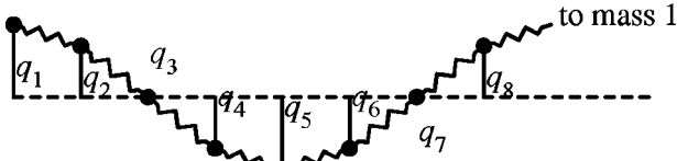
Fig. 8. The eight-particle system of harmonic oscillators connected by springs of spring constant \kappa . All masses are constrained to move vertically along the coordinates q_1 through q_8 . Mass 8 is connected by a spring to mass 1, as if the masses were arranged in a ring, giving periodic boundary conditions.
