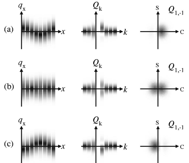
Fig. 17. Time sequence for the quantum mechanical lattice in a superposition of states, the ground state and a one-phonon state, 1/\sqrt{2}[\hat{A}_1^\dagger|0\rangle + |0\rangle] .
