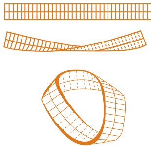
Forming a Möbius strip
