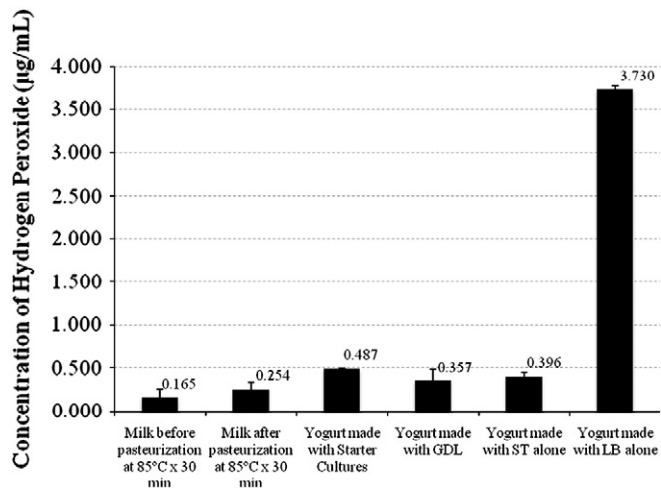
Fig. 5. Hydrogen peroxide content ( \mu\text{g/mL} ) in pre- and post-pasteurized reconstituted non-fat dry milk, and different types of yogurt. S. thermophilus and L. delbrueckii ssp. bulgaricus are abbreviated as [ST] and [LB], respectively.
