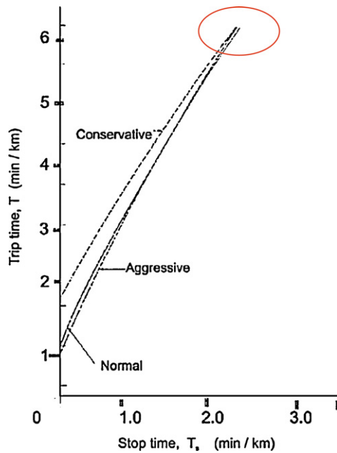
Fig. 2. The two fluid trends for aggressive, normal and conservative drivers in the Austin CBD (Herman et al., 1988).
