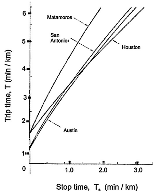
Fig. 1. Two-fluid model for various cities (Herman and Ardekani, 1984).
