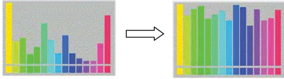
Figure 3 - Histogram equalization
