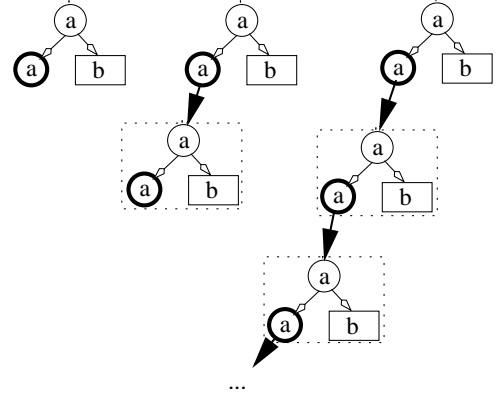
Figure 7. ECRrecognizer on content of \langle a \rangle in the XML string \langle a \rangle \langle b \rangle \langle /b \rangle \langle b \rangle \langle /b \rangle \langle /a \rangle and DTD T_1 from Example 5
