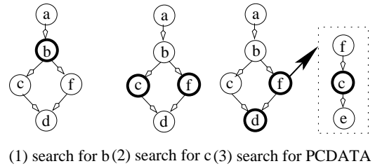
A. ECR recognizer on string w: b, e, c, PCDATA
