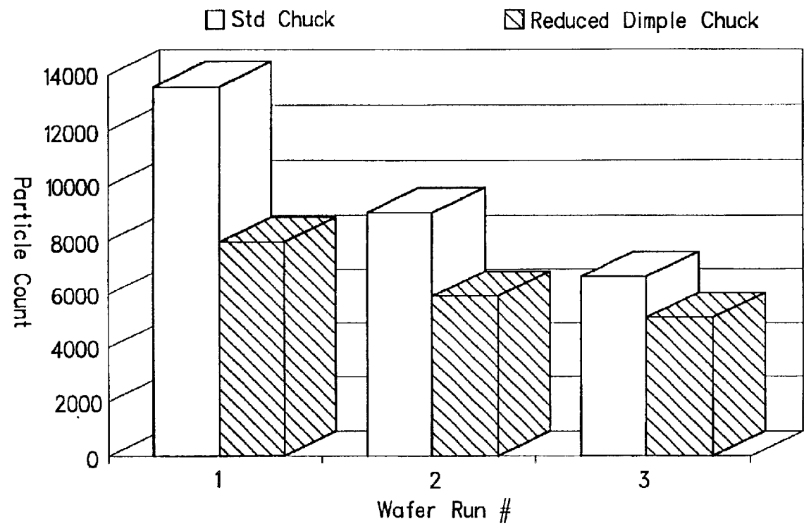
Standard Chuck vs Reduced Dimple Chuck
