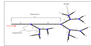
Figure 4. Schematic of the Strahler ordering scheme.
