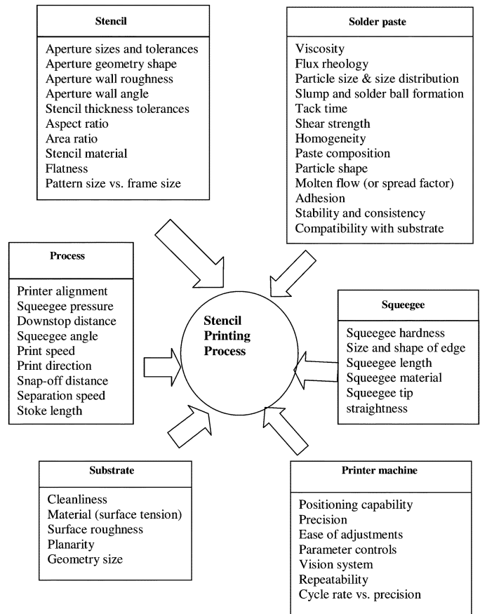
Fig. 1. Factors that influence the stencil printing process.
