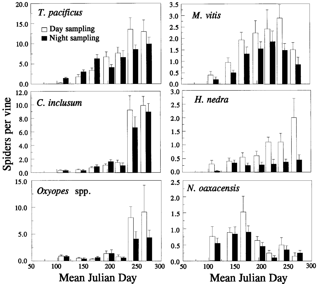
Figure 1.—Spidedensity per vine of the six most common taxa, 1993 and 1994 data combined, with the julian dates of the two study years averaged. Open bars represent day sampling, and closed bars night sampling. Metaphidippus vitis and H. nedra showed significantly higher density with day sampling ( P < 0.01 ). No significant differences were found in spider density for any of the other taxa.
