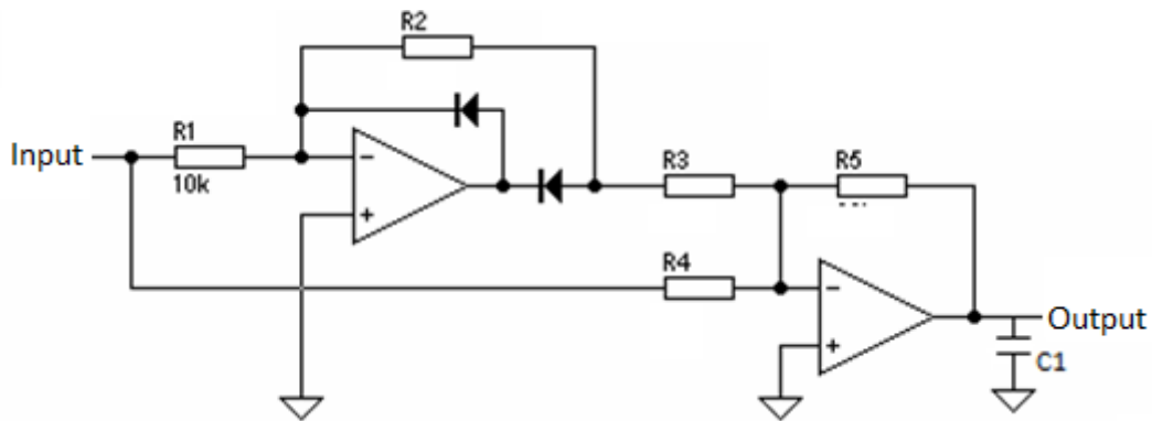
Full Wave Rectifier Figure 6
