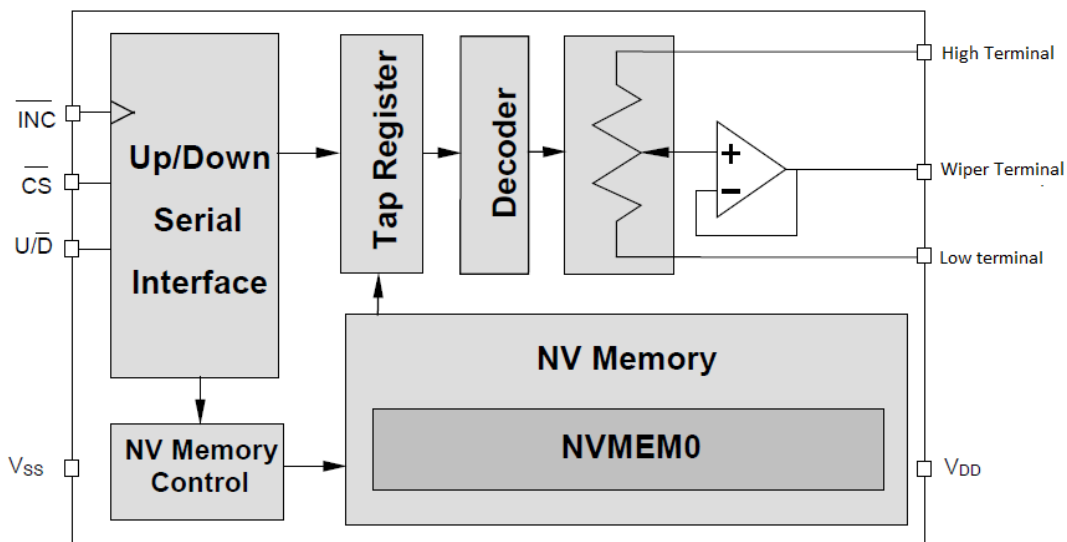
WMS7170 Digital Potentiometer Modified from WMS7170 datasheet Figure 7
