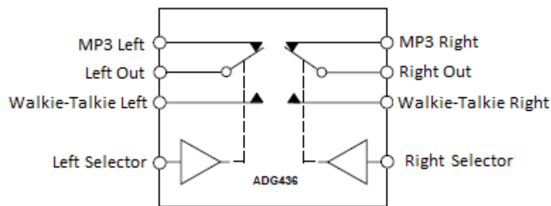
ADG436B Analog Switch Figure 3
