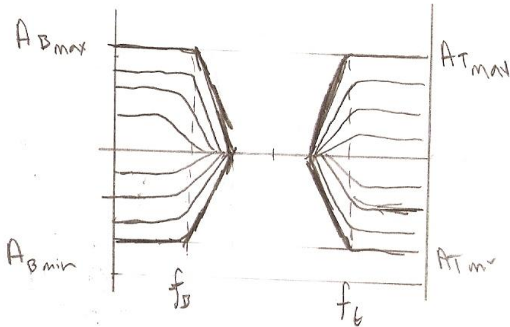
Frequency response of equalizer (Franco) Figure 5
