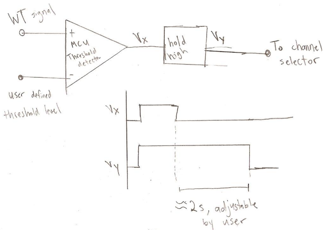
Conceptual functionality of microcontroller comparator
