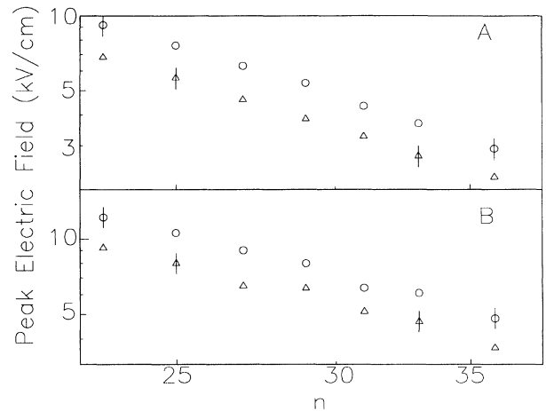
FIG. 4. Peak HCP field required to ionize (A) 10% and (B) 50% of the Rydberg population as a function of n for a (O) “clean” pulse and ( \Delta ) “unclean” pulse. Significantly attenuating the imperfections in the pulse increases the requisite fields by a factor of 1.3.
