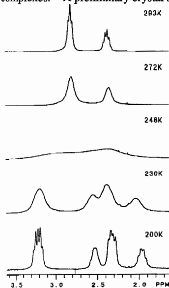
Figure 3: 300 MHz ^1H NMR spectrum of TC_5 TPP dication as a function of temp.
